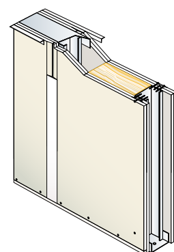
Exemple de cloison distributive
